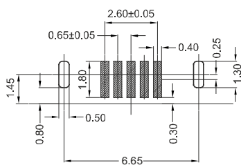
RECOMMENDED PCB LAYOUT Tolerance \pm 0.05
